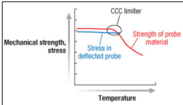
Figure 3 Mechanical strength of typical spring metals diminishes rapidly past critical temperature, marked here as “CCC limiter.”
