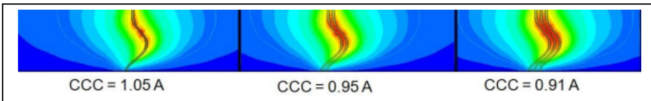
Figure 4 Influence of neighboring probe proximity on CCC at 130µm pitch. Color indicates temperature distribution. Red shows maximum allowable temperature. Plots achieved through FEA were confirmed through measurement.
