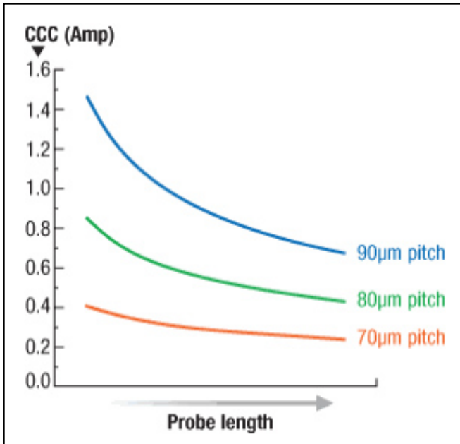
Figure 5 Example relationship between probe CCC and probe length for geometries allowing 70, 80, and 90µm pitch in full grid array chip layouts. Note that the shortest probes here might not provide sufficient deflection for applications with large system planarity.
