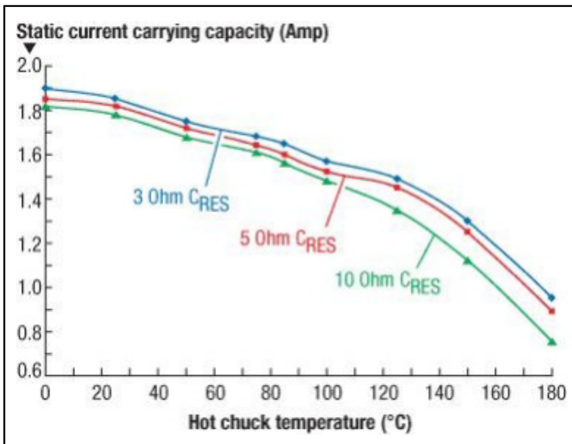
Figure 2 Figure 2. CCC as a function of wafer temperature and contact resistance. Data for 75µm probe deflection.
