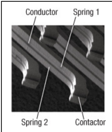
Figure 8 Composite micro electromechanical system (MEMS) structure of MicroProbe Vx-RF probe optimizes conductivity, strength at elevated temperature and contact resistance performances
