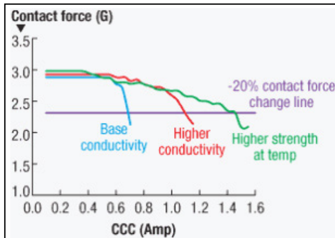
Figure 1 Typical plot resulting from the SEMI methodology; a 20% contact force reduction marks the CCC spec. CCC improvement achieved through probe material conductivity (electrical and thermal) and high temperature strength increase. 75µm probe deflection.
