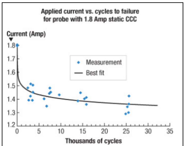
Figure 7 Example of dynamic CCC test result correlating current to number of achievable probing cycles for a probe with 1.8Amp static CCC.
